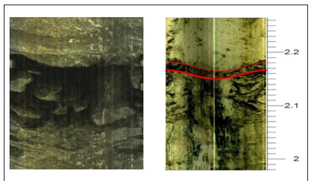
Borehole image of a shatter zones
